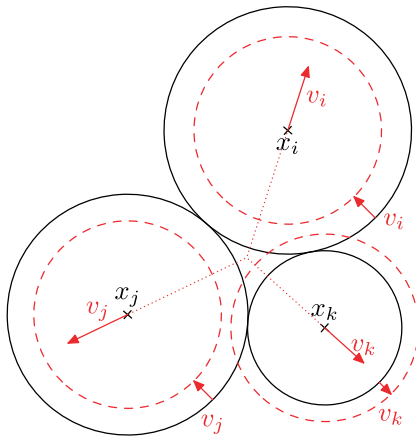
Fig. 3. A cluster with three globules and the associated impulsion \mathbf{v}(\mathbf{x}) constructed to push \mathbf{x} \in \partial\mathcal{D} back into the interior of the set of allowed globule configurations.
