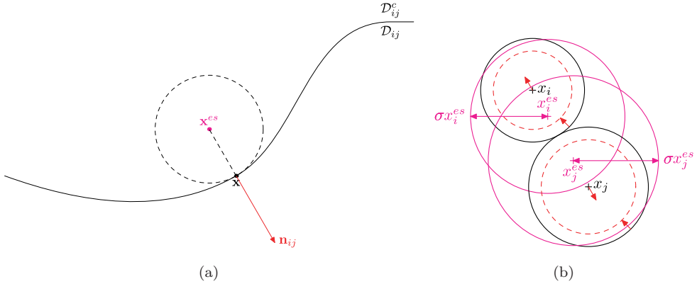
Fig. 2. A configuration \mathbf{x} \in \partial\mathcal{D}_{ij} and the corresponding center \mathbf{x}^{es} of the uniform exterior sphere : \mathbf{x}^{es} = \mathbf{x} - \alpha_{ij}\mathbf{n}_{ij}(\mathbf{x}) = \mathbf{x} - r_-\sqrt{2+2\sigma^2}\mathbf{n}_{ij}(\mathbf{x}) . (a) a simplified representation in \mathbb{R}^2 . (b) a representation as a pair of colliding globules. Remark that \mathbf{x}^{es} \notin \mathcal{A}_g^\sigma .
