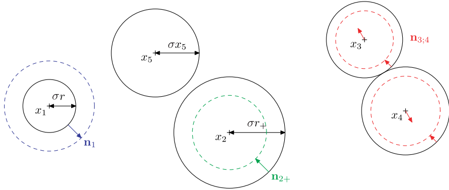
Fig. 1. A configuration of five globules in \partial\mathcal{D}_{1-} \cap \partial\mathcal{D}_{2+} \cap \partial\mathcal{D}_{3;4} \cap \mathcal{A}_g^\sigma , and the different directions of impulsion \mathbf{n}_{1-} , \mathbf{n}_{2+} or \mathbf{n}_{3;4}(\mathbf{x}) to go back into the interior of \mathcal{A}_g^\sigma .
